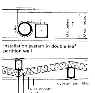
⑮ Noise insulating double-leaf wall construction
